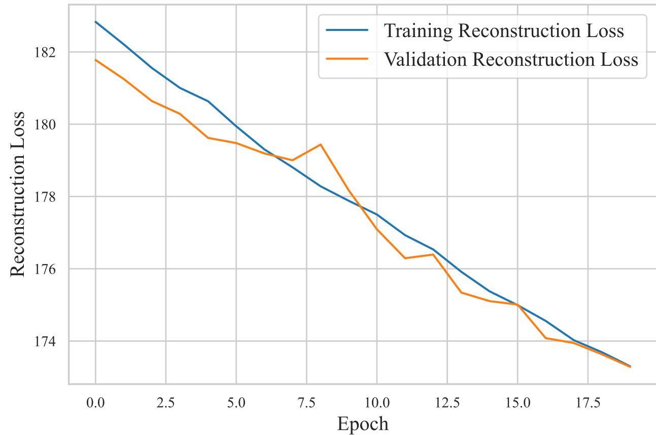
VAE: Reconstruction Loss
